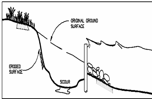
EROSION BEHIND STRUCTURE - WAVES LAP OVER TOP SIDE VIEW
