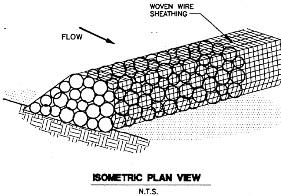
Figure 3-23 Schematic Diagram of a Rock Berm
