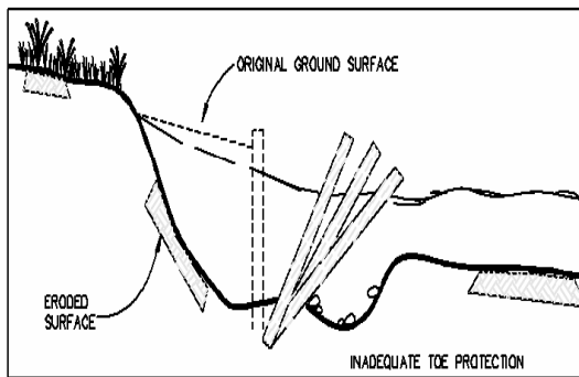
SLUMPING DUE TO TOE SCOUR SIDE VIEW
