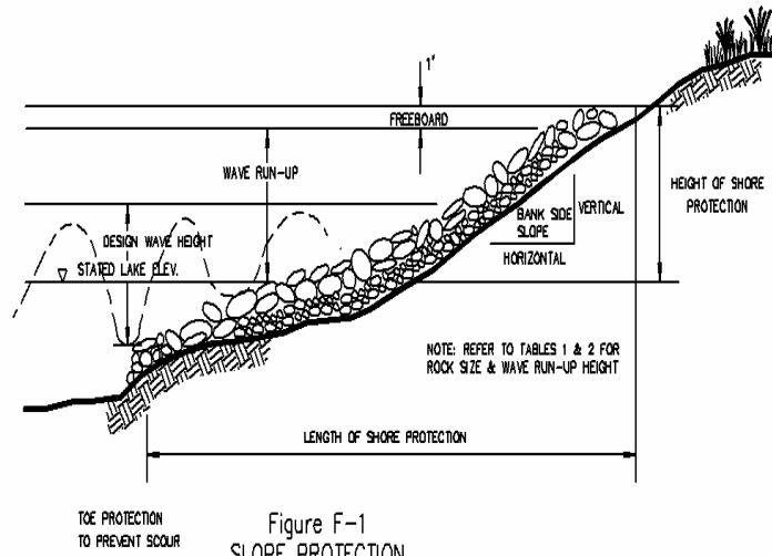
Figure 6-1 Slope Protection Using Rock Riprap
