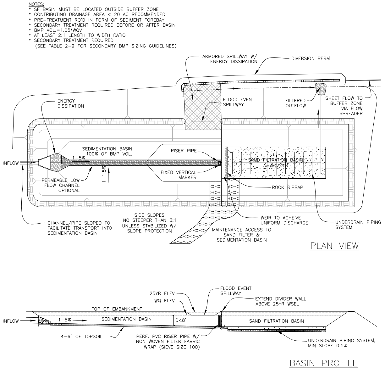
Figure 4-3: Sand Filter System Schematic
