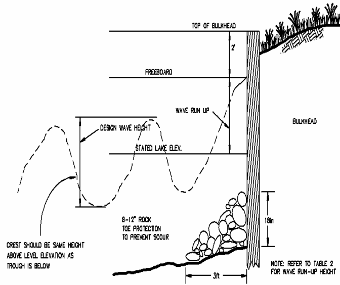
Figure F-2 VERTICAL PROTECTION USING RETAINING WALL
