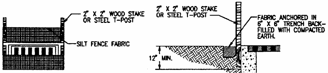
Figure 3-27 Filter Fabric Inlet Protection
