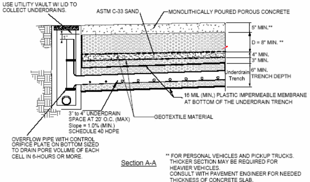
Figure 4.19: Schematic of Permeable Concrete with Underdrain Installation (after UCFCD, 2004)
