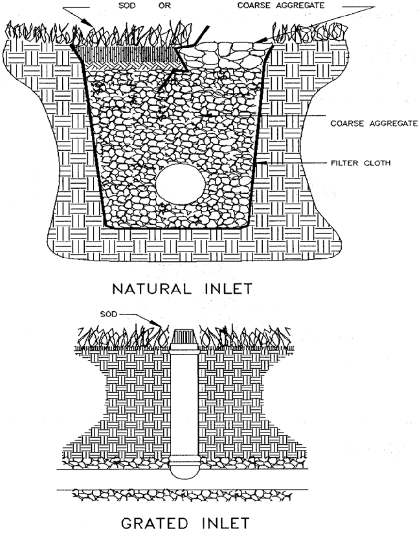
Figure 3-10 Surface Inlets for Subsurface Drains
