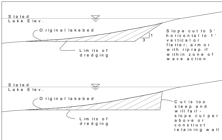
FIGURE F-5 CUT SLOPE FOR DREDGED AREA
